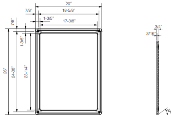
ALM03FF - Front Wall Mount
