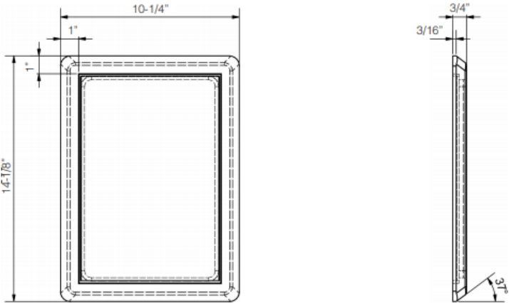
ALM02 - Through Wall Mount
