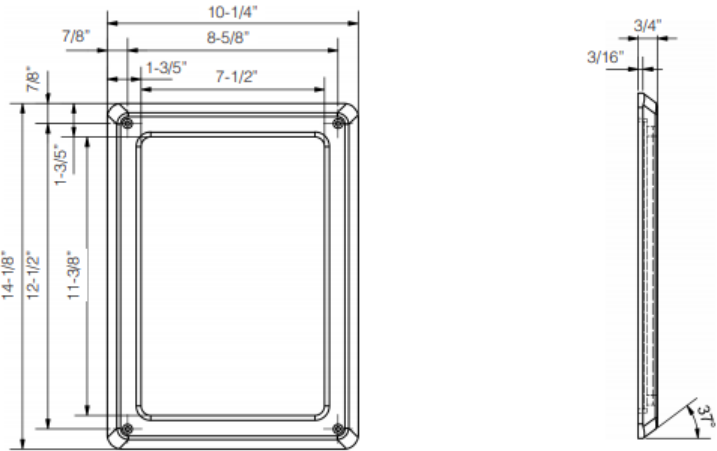
ALM02 - Front Wall Mount
