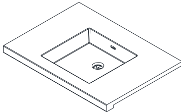
-BBSQ SQUARE BASIN 14" W x 14" L x 4" D Basin (356mm x 356mm x 102mm)
