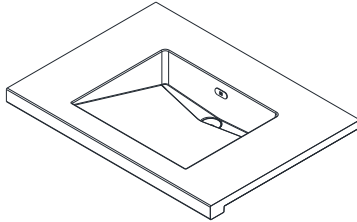
-BBED SLOPED BASIN 16-3/4" W x 13-3/4" L x 4" D Basin (425.5mm x 349mm x 102mm)
