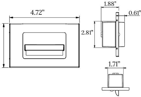
HORIZONTAL HOOD
