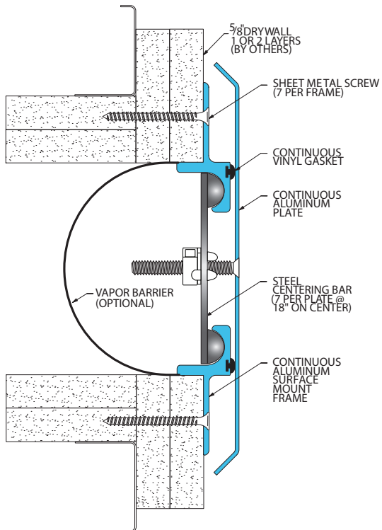
Vapor Barrier System (491-A07-100 system shown)
