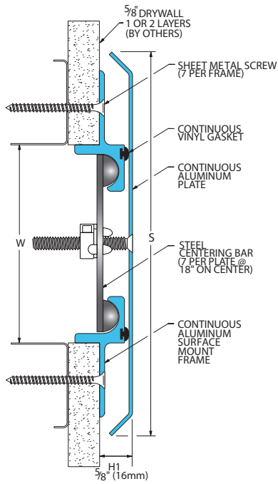
491-A07 Wall/Wall, Ceiling/Ceiling (4" (100mm) system shown)
