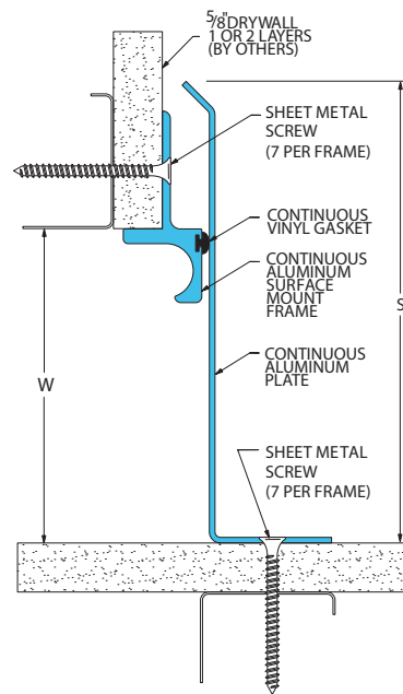
491-A09 Wall/Corner, Wall/Ceiling (4" (100mm) system shown)
