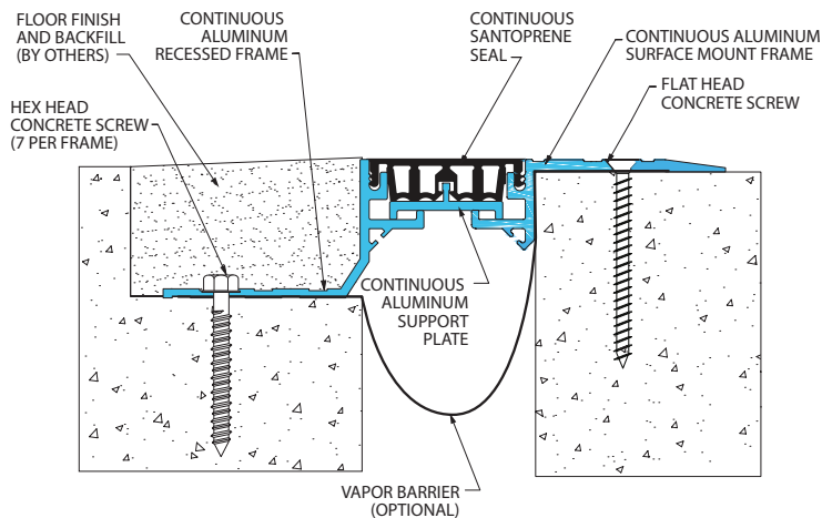
Vapor Barrier (107-A01-050 system shown)
