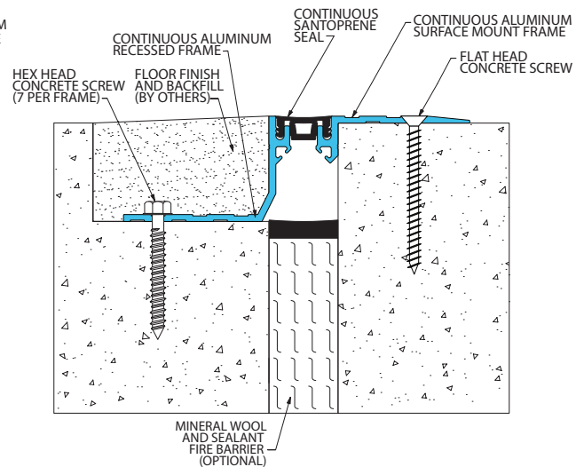
Fire Barrier (107-A01-025 system shown)
