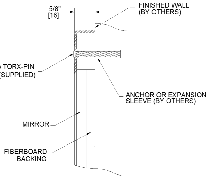
INSTALLATION DETAIL
